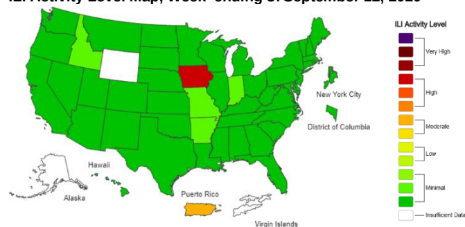
ILI Activity Level Map, Week ending 37 September 12, 2020
